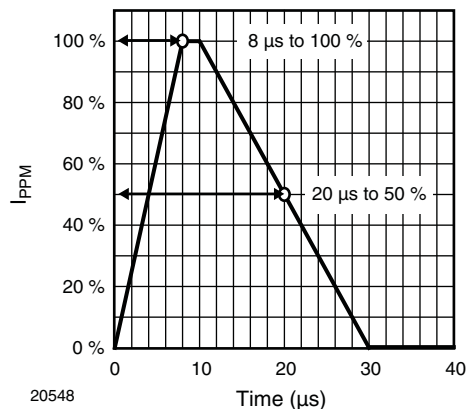
Fig. 1 - 8/20 \mu\text{s} Peak Pulse Current Wave Form acc. IEC 61000-4-5
