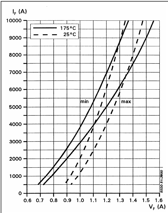
Fig. 2 On-state characteristics.
