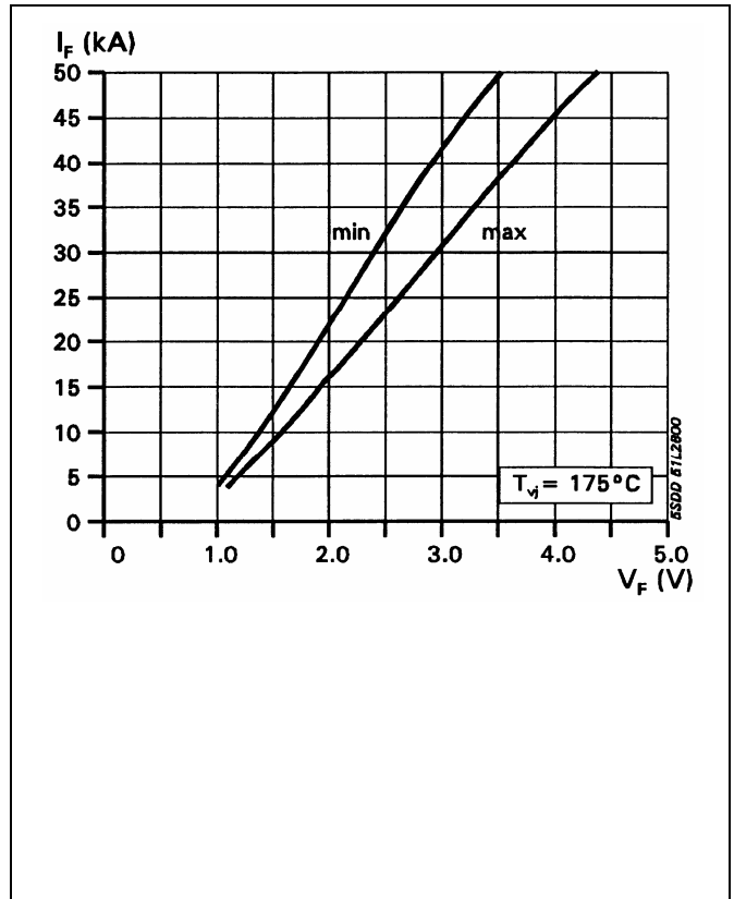
Fig. 3 On-state characteristics.
