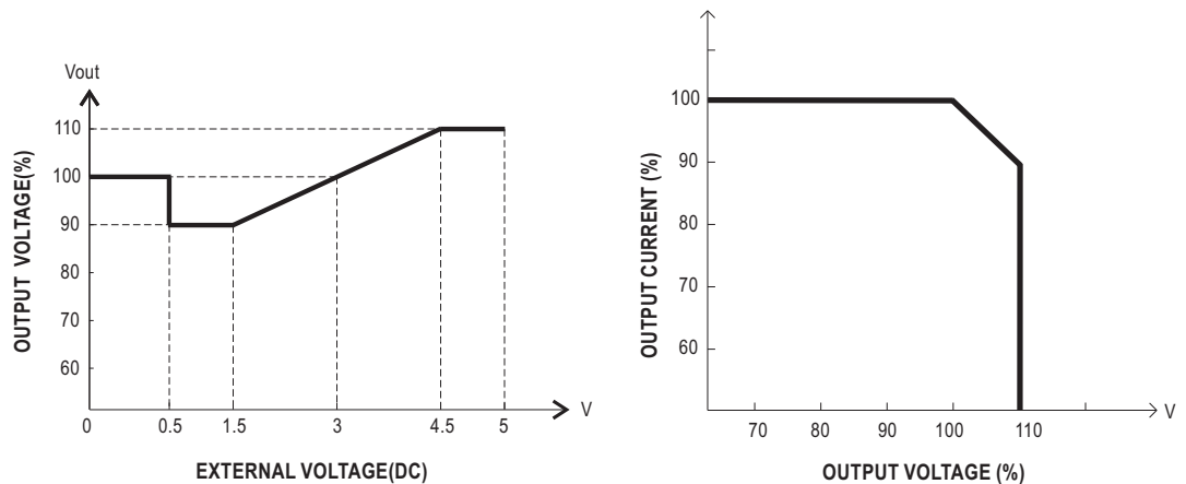
Fig. 3.2 Output voltage trimming
