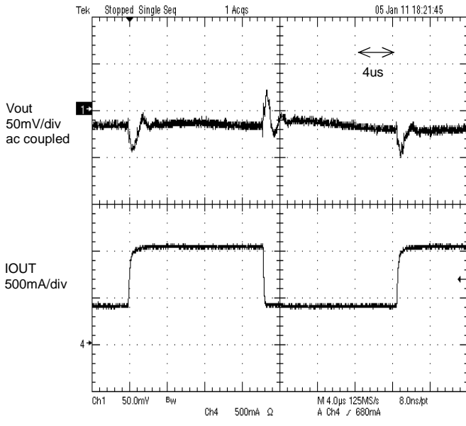
Figure 21. Load transient response 400mA to 100mA tr=tf=100ns, MODE : Low
