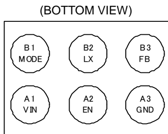
Figure 2. Pin Configuration(s)
