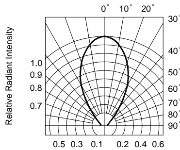
FIG.6 RADIATION DIAGRAM
