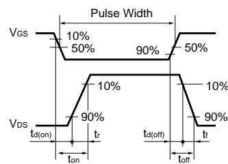
Fig.3-2 Switching Waveforms
