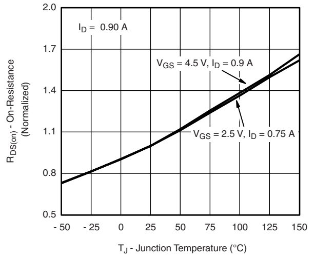
I_D = 0.90\text{ A} V_{GS} = 4.5\text{ V}, I_D = 0.9\text{ A} V_{GS} = 2.5\text{ V}, I_D = 0.75\text{ A} On-Resistance vs. Junction Temperature
