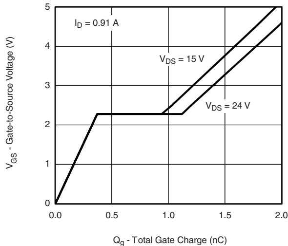
I_D = 0.91\text{ A} V_{DS} = 15\text{ V} V_{DS} = 24\text{ V} Gate Charge
