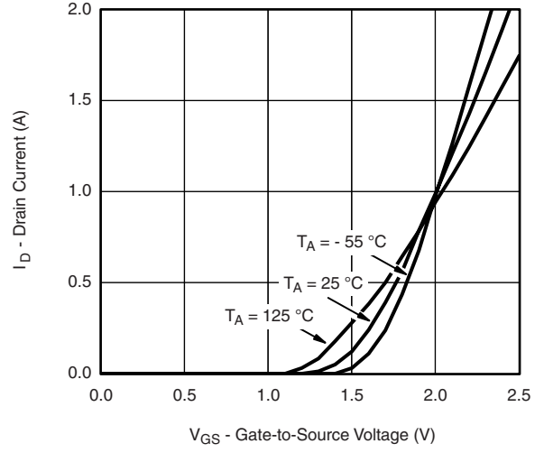
T_A = -55\text{ }^\circ\text{C} T_A = 25\text{ }^\circ\text{C} T_A = 125\text{ }^\circ\text{C} Transfer Characteristics Curves vs. Temperature
