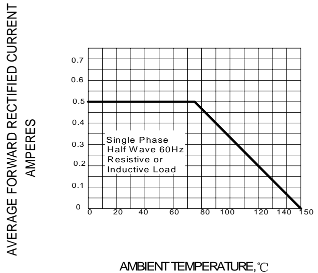
FIG.3 – FORWARD DERATING CURVE
