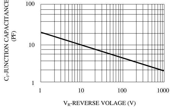
FIG. 6-TYPICAL JUNCTION CAPACITANCE
