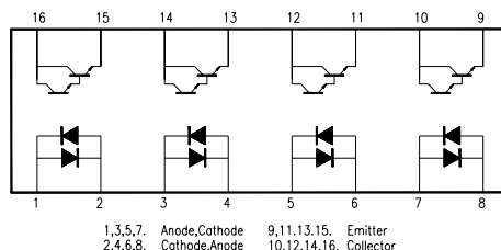
1,3,5,7. Anode,Cathode 9,11,13,15. Emitter 2,4,6,8. Cathode,Anode 10,12,14,16. Collector
