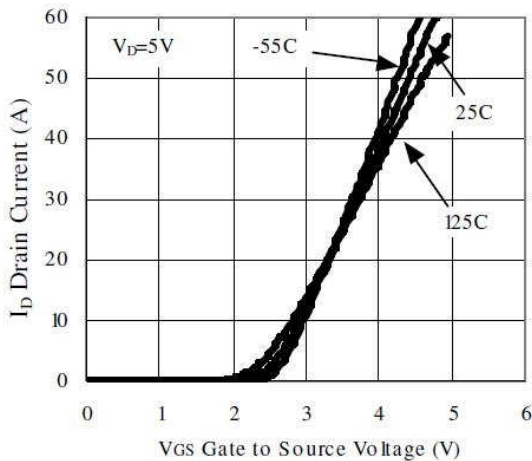
Figure 5. Transfer Characteristics
