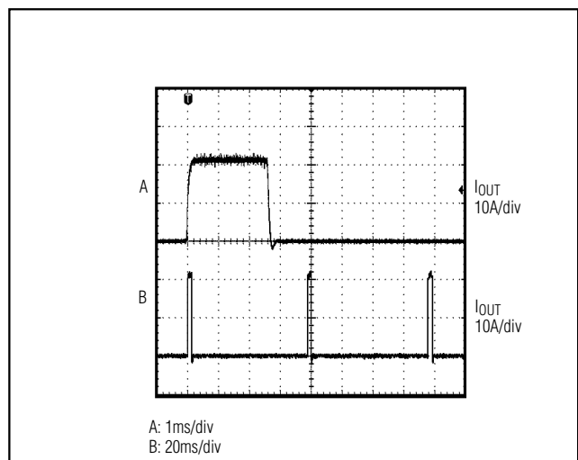
Figure 8. Load Current (10A/div) as a Function of Time when Converter Attempts to Turn On into a 0.050Ω Short Circuit (Also Acts as Current-Sense Resistor)
