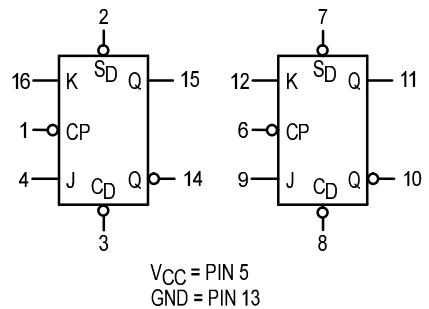
LOGIC SYMBOL
