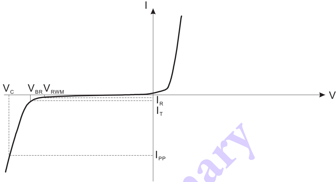
Uni-Directional TVS
