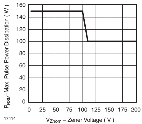
Figure 4. Maximum Pulse Power Dissipation vs. Zener Voltage
