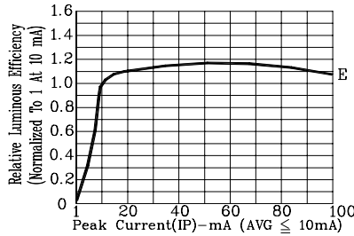
Fig2. RELATIVE LUMINOUS EFFICIENCY (LUMINOUS INTENSITY PER UNIT CURRENT) VS. PEAK CURRENT (REFRESH RATE 1KHz)
