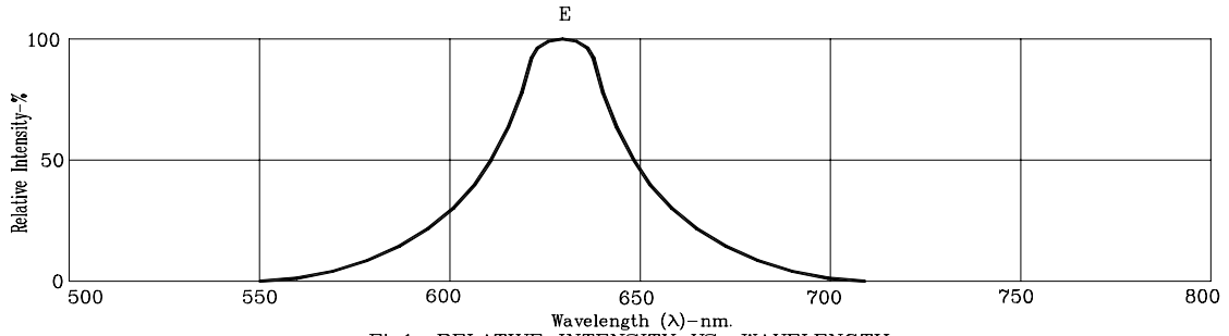
Fig1. RELATIVE INTENSITY VS. WAVELENGTH
