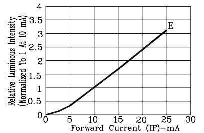
Fig4. RELATIVE LUMINOUS INTENSITY VS. FORWARD CURRENT
