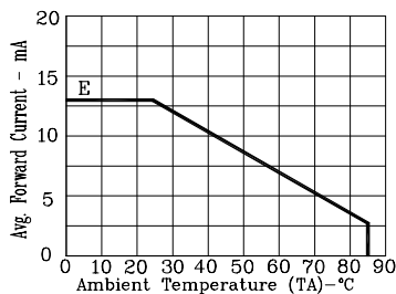
Fig5. MAX. AVERAGE FORWARD CURRENT VS. AMBIENT TEMPERATURE.
