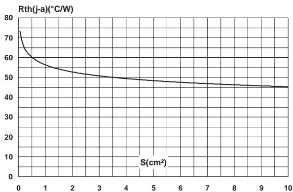
Fig. 8: Thermal resistance junction to ambient versus copper surface under each lead (epoxy printed board FR4, Cu = 35µm).
