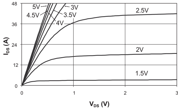
Output Characteristics
