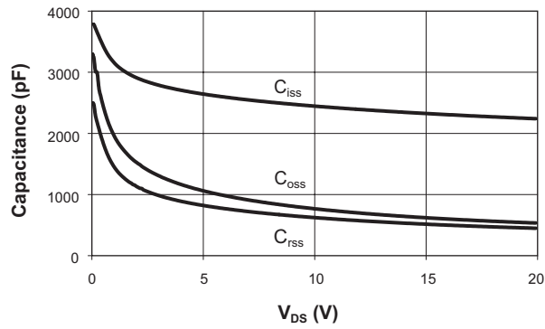
Capacitance
