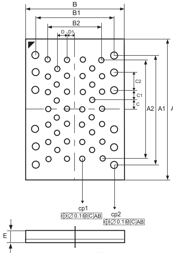
Figure 38: 52-ULGA, 12 x 17mm, Package Outline (Top view through package)
