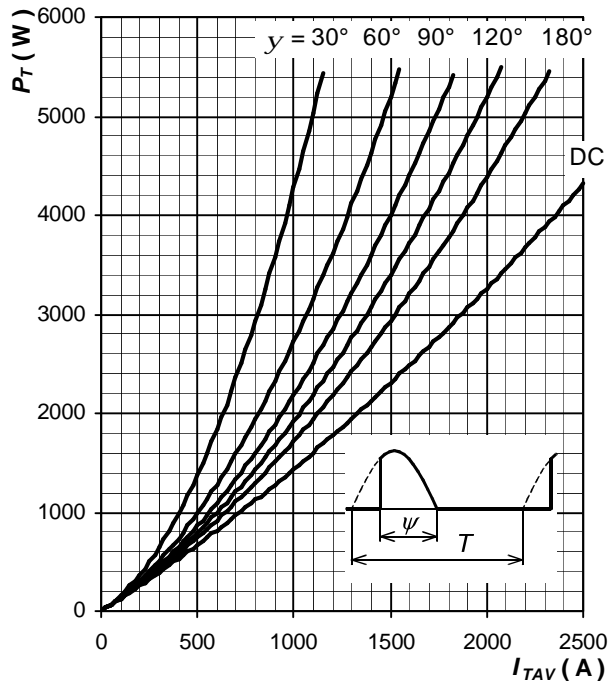
Fig. 5 On-state power loss vs. average on-state current, sine waveform, f = 50 Hz, T = 1/f
