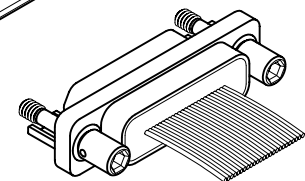
KEYING JACKSCREW – KS (100 POSITION = KJ)
