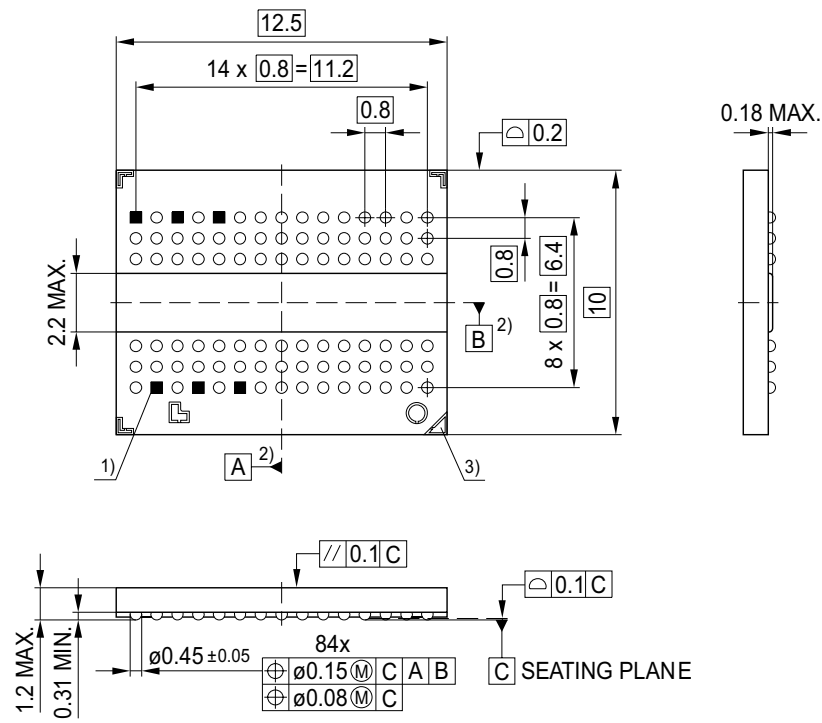
FIGURE 13 Package Outline PG-TFBGA-84
