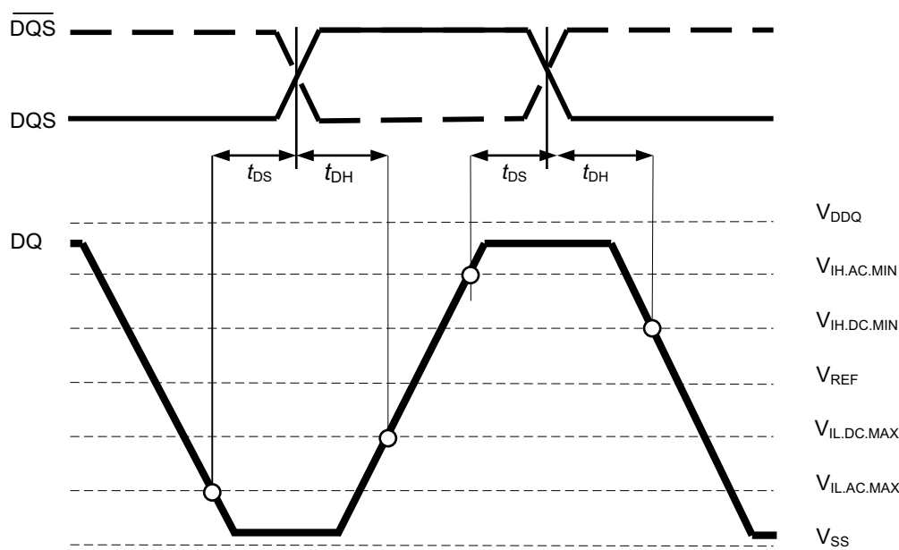
Differential Input Waveform Timing - t_{DS} and t_{DH}
