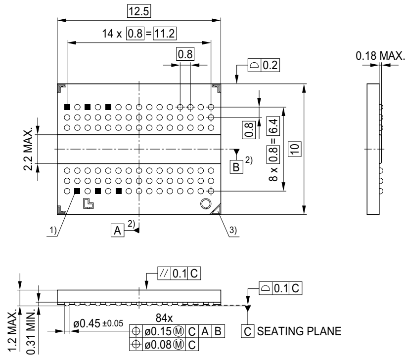
FIGURE 12 Package Outline P-TFBGA-84
