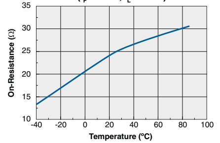
Typical On-Resistance vs. Temperature ( I_F=10mA, I_L=80mA )
