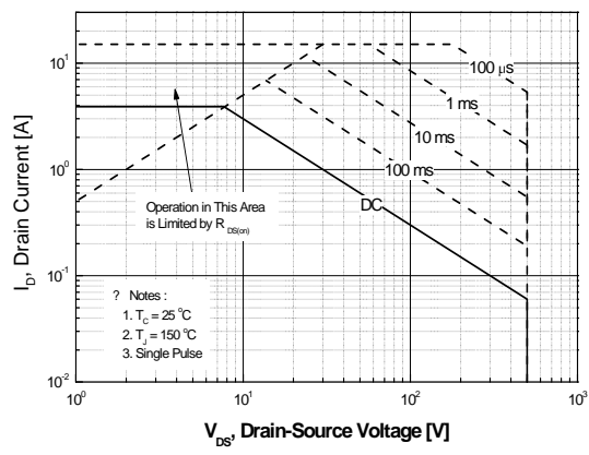
Figure 8. Maximum Safe Operating Area vs. Case Temperature-FDPF5N50NZU
