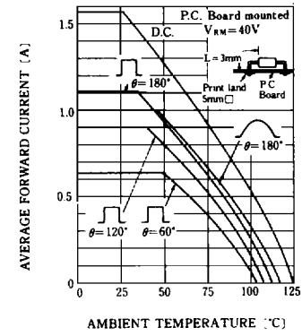
FIG.6-AVERAGE FORWARD CURRENT VS. AMBIENT TEMPERATURE
