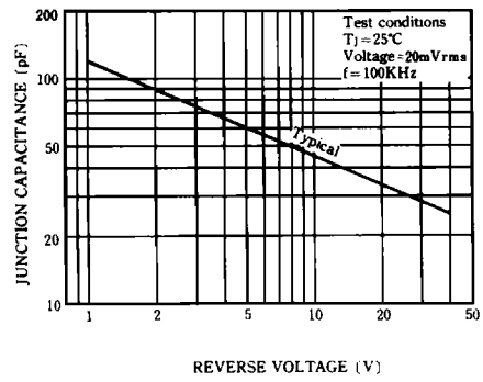
FIG.8-JUNCTION CAPACITANCE VS. REVERSE VOLTAGE
