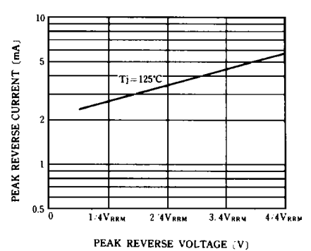
FIG.3-PEAK REVERSE CURRENT VS. PEAK REVERSE VOLTAGE
