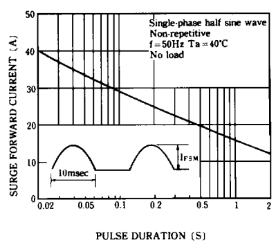
FIG.7-SURGE CURRENT RATINGS
