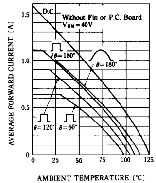
FIG.5-AVERAGE FORWARD CURRENT VS. AMBIENT TEMPERATURE
