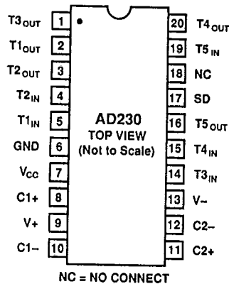
Figure 1. AD230 DIP/SOIC Pin Configuration
