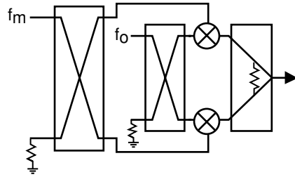
SDM, SML-A...D Single-Sideband Upconverter LO and 1/2 LO
