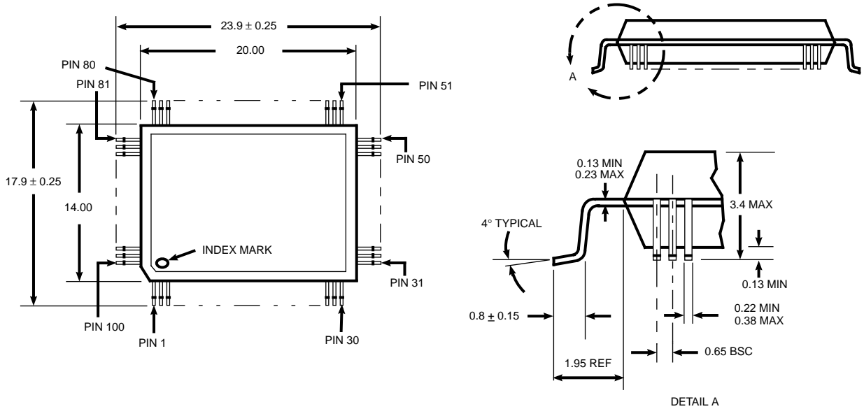
Figure 7. FAS236/236U 100-Pin PQFP Mechanical Drawings
