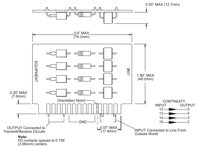
TEL185B BOARD OUTLINE
