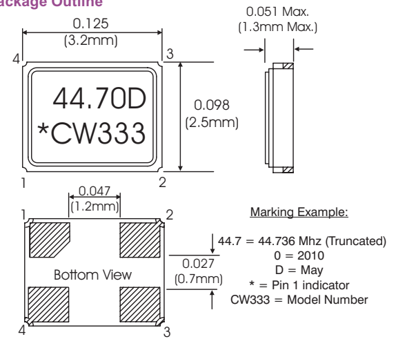
Marking drawing 90231DWG74
