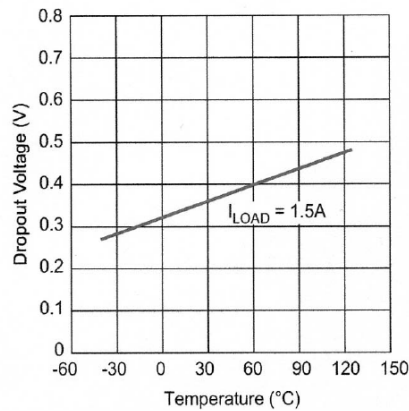
LM27150 Dropout Voltage vs. Temperature
