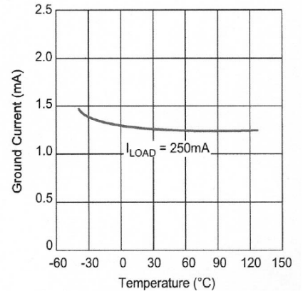
LM27150 Ground Current vs. Temperature
