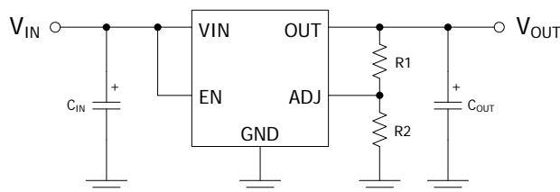
Figure 2. Adjustable Regulator with Resistors
