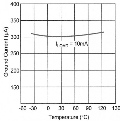
LM27150 Ground Current vs. Temperature
