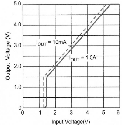
LM27150-5.0 Dropout Characteristics
