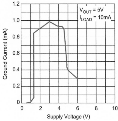
LM27150 Ground Current vs. Supply Voltage
