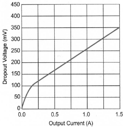
LM27150 Dropout Voltage vs. Output Current
