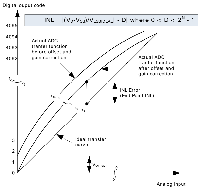
Figure 3.12. Integral Non-Linearity (INL)
