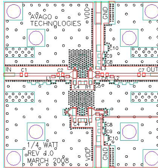
Figure 44. Demoboard
