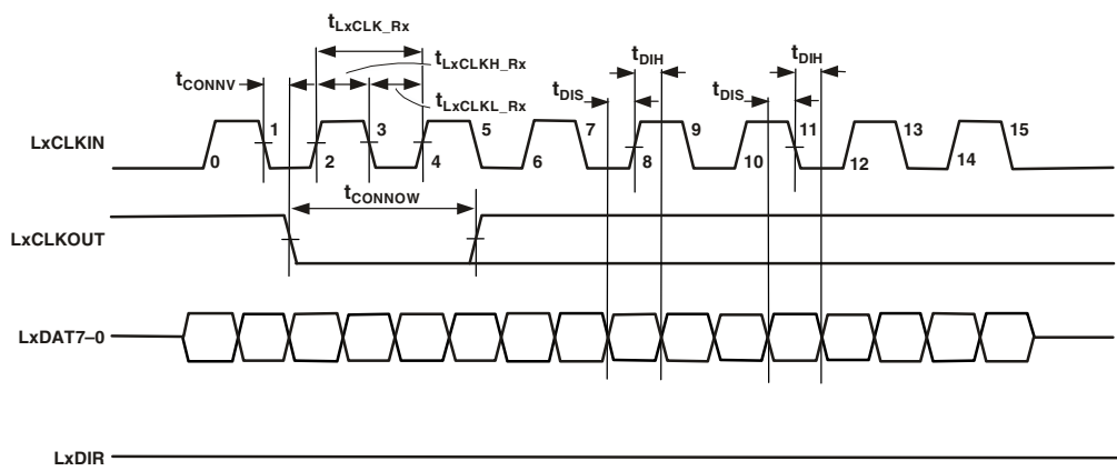
Figure 18. Link Ports—Receive
