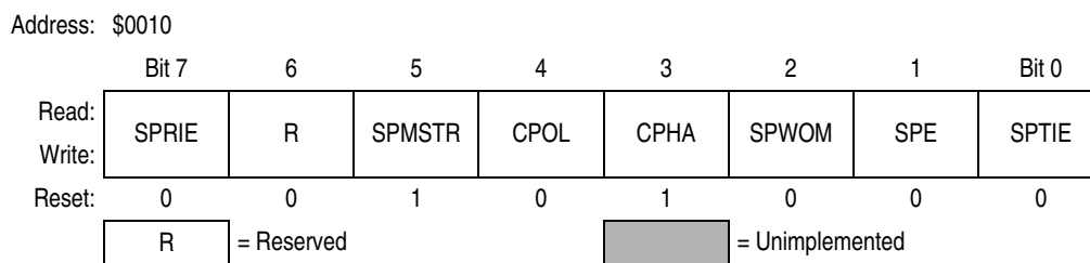
Figure 17-14. SPI Control Register (SPCR)
