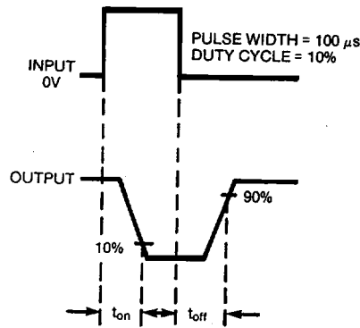
Fig. 11. Switching Time Waveforms
