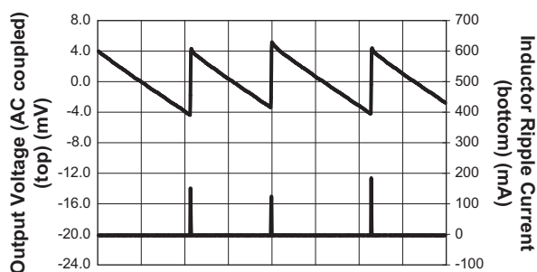
Light Load Switching Waveform (Light-Load Mode; V_{IN} = 3.6V ; V_{OUT} = 1.8V ; 1mA Load)
