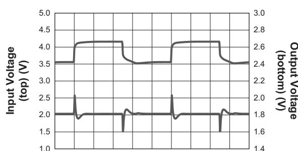
Line Transient Response ( V_{OUT} = 1.8V ; 1.5A Load)
