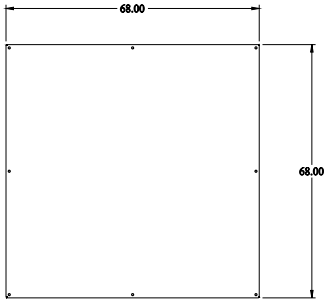
INNER PANEL
