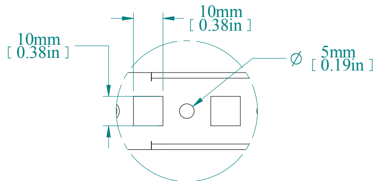
DETAIL A
