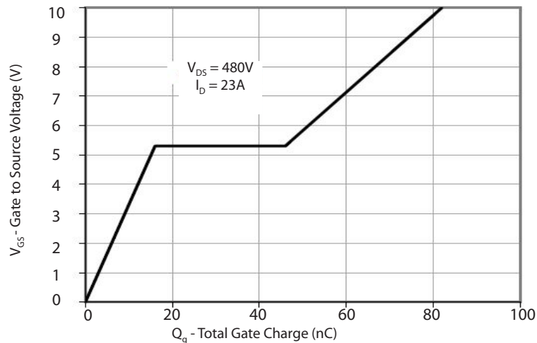
Gate Charge
