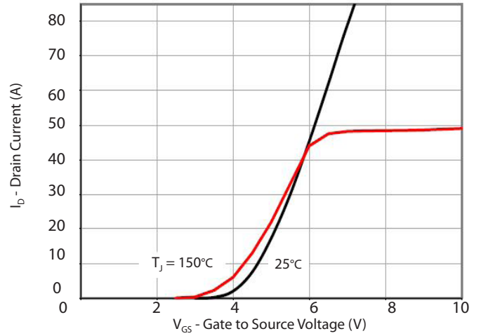
Transfer Characteristics
