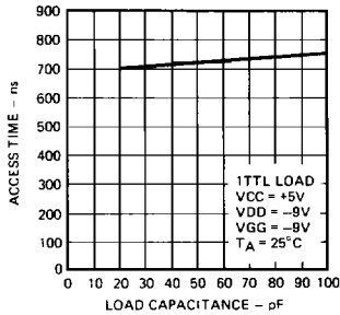
Access Time Versus Load Capacitance
