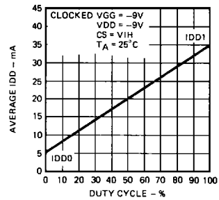
Average Current Versus Duty Cycle for Clocked VGG
