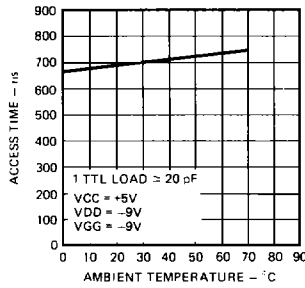
Access Time Versus Temperature
