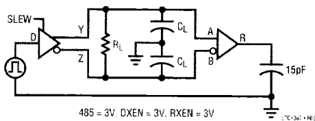
Figure 2. RS485 Driver/Receiver Timing Test Circuit
