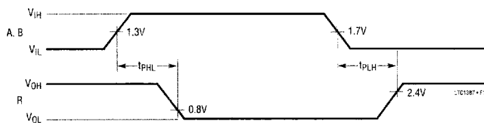
Figure 11. RS232 Receiver Propagation Delays
