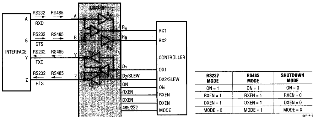
Figure 16. Full-Duplex RS232 (2-Channel), Full-Duplex RS485/RS422 with SLEW Control
