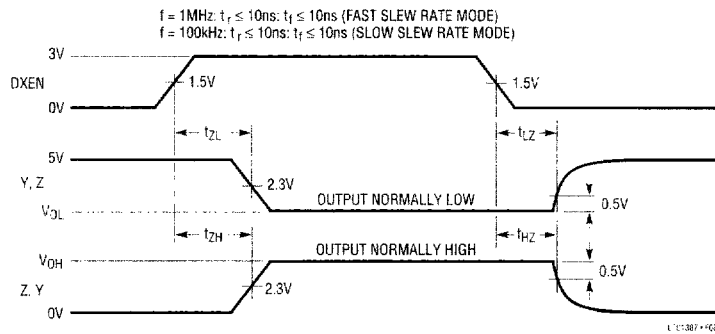
Figure 8. RS485 Driver Enable and Disable Times
