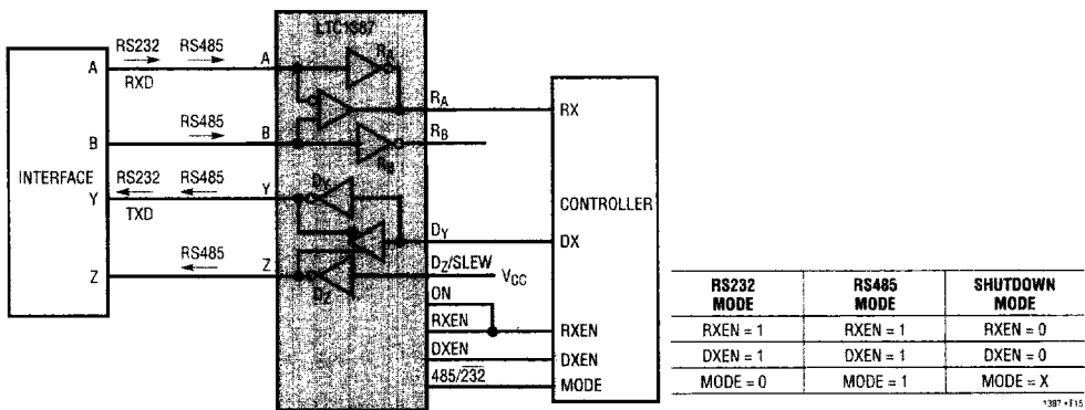
Figure 15. Full-Duplex RS232 (1-Channel), Full-Duplex RS485/RS422
