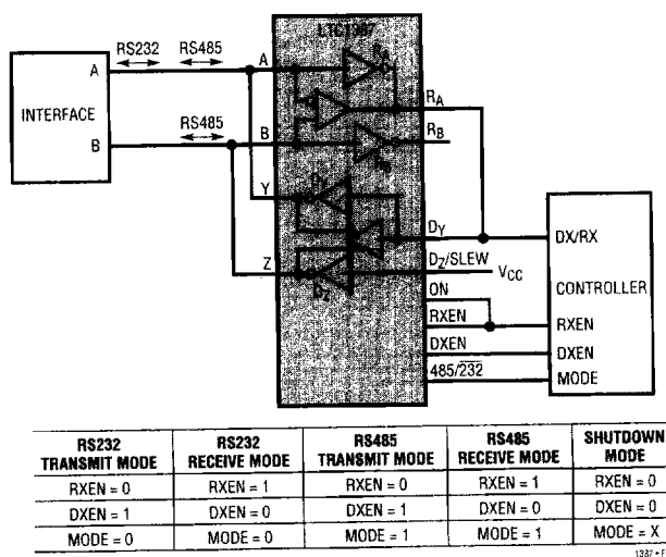
Figure 13. Half-Duplex RS232 (1-Channel), Half-Duplex RS485
