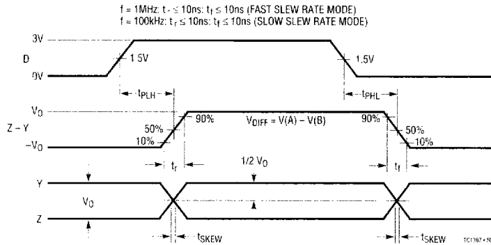
Figure 7. RS485 Driver Propagation Delays
