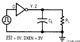
Figure 4. RS232 Driver Timing Test Circuit
