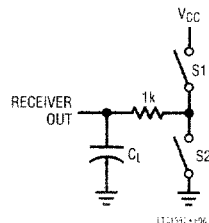
Figure 6. Receiver Output Enable/Disable Timing Test Load
