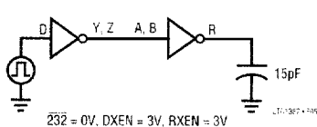
Figure 5. RS232 Receiver Timing Test Circuit
