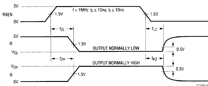
Figure 12. Receiver Enable and Disable Times
