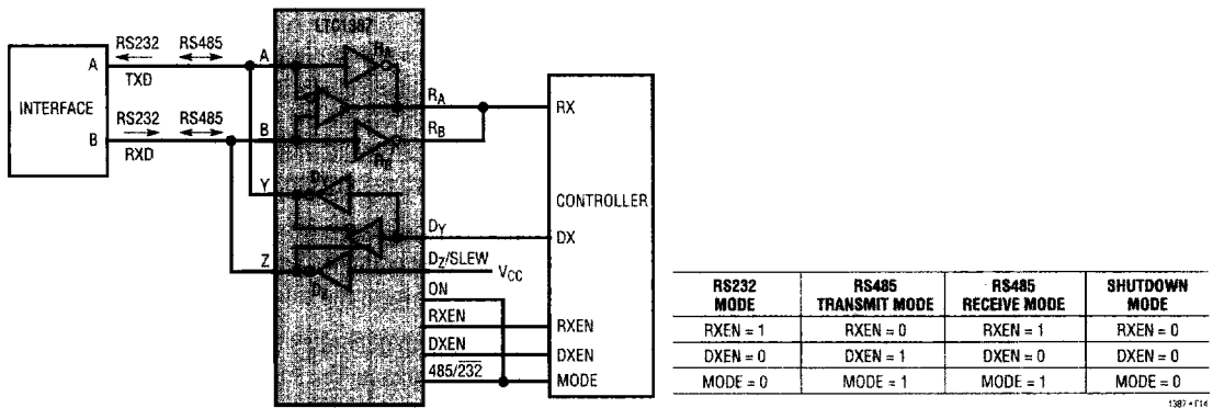
Figure 14. Full-Duplex RS232 (1-Channel), Half-Duplex RS485
