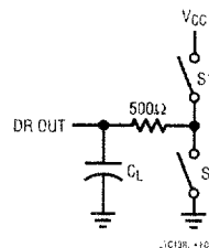
Figure 3. RS485 Driver Output Enable/Disable Timing Test Load
