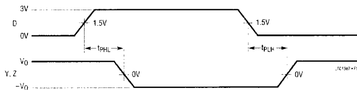
Figure 10. RS232 Driver Propagation Delays
