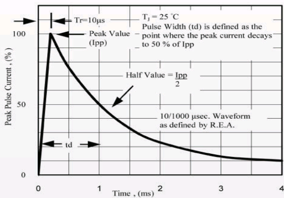
Fig. 5 - Pulse Waveform
