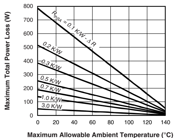
Fig. 9 - Forward Power Loss Characteristics
