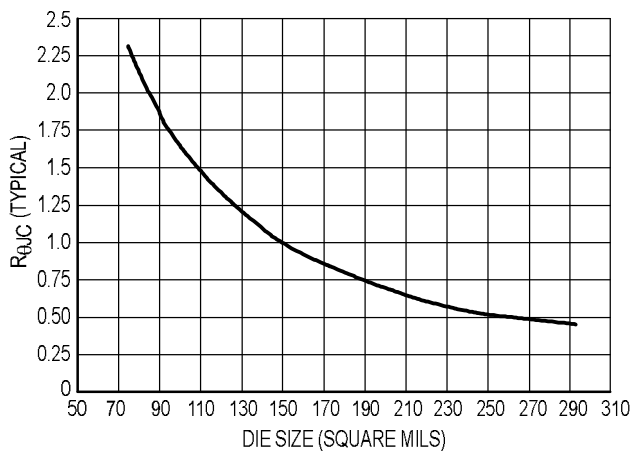
Figure 5. R_{\theta JC} versus Die Size for TMOStm Devices in TO-220, D2PAK, DPAK & TO-247 Packages
