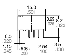
2 coil latching
