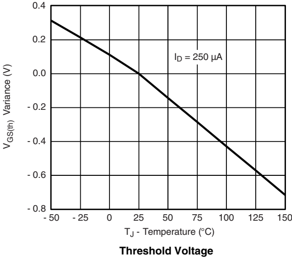
Threshold Voltage
