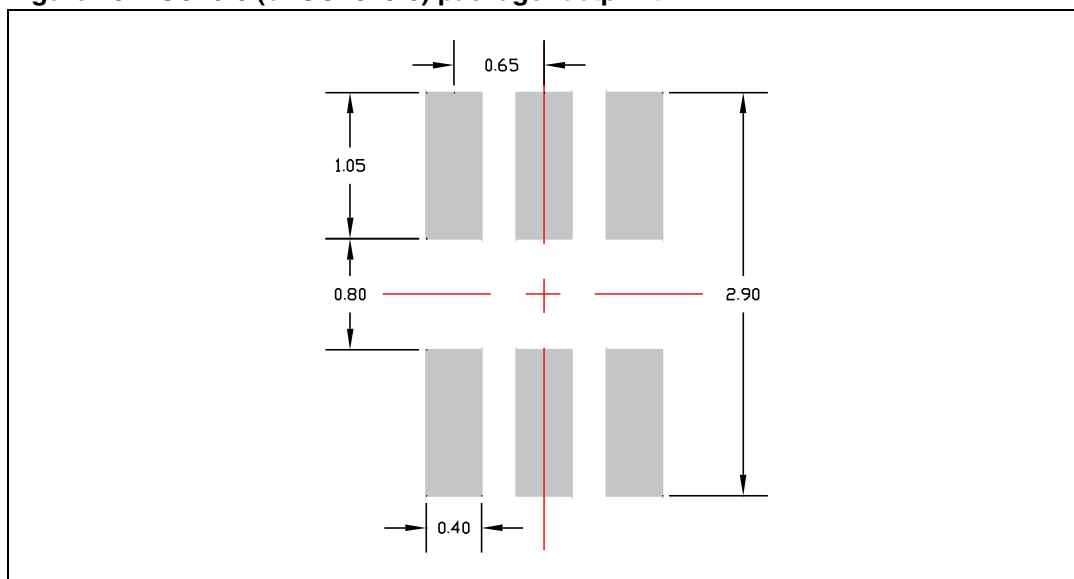
Figure 23. SC70-6 (or SOT323-6) package footprint
