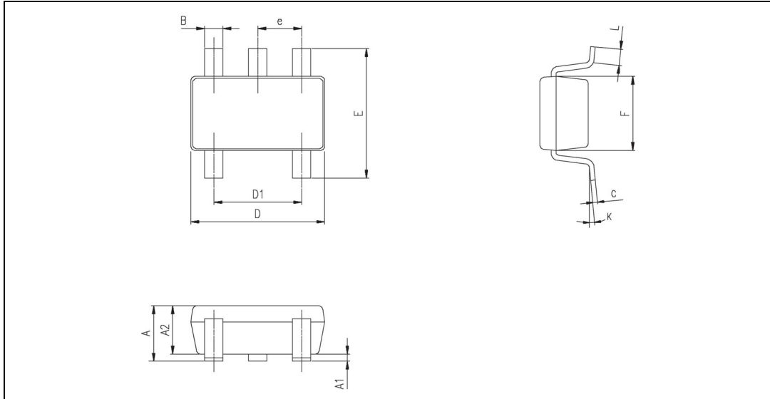
Figure 19. SOT23-5L package mechanical drawing
