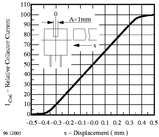
Figure 10. Rel. Collector Current vs. Displacement
