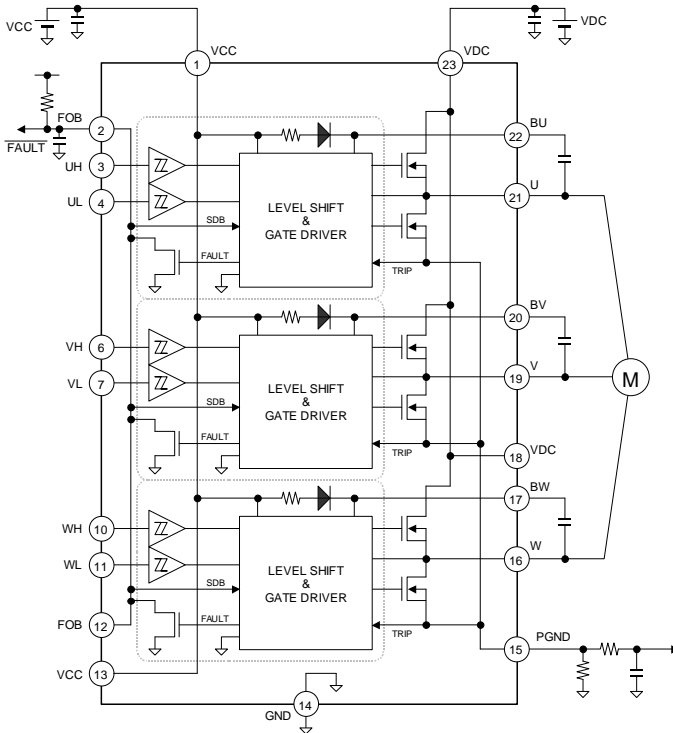
Figure 2. Block Diagram
